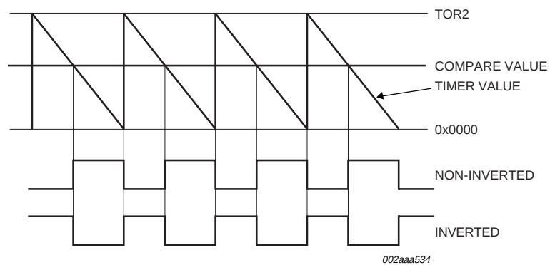
Fig 15. Asymmetrical PWM, downcounting.
