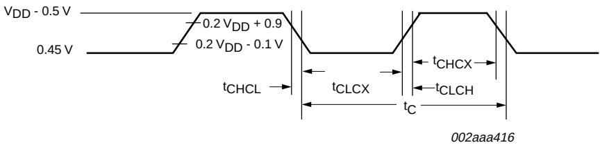
Fig 29. External clock timing.
