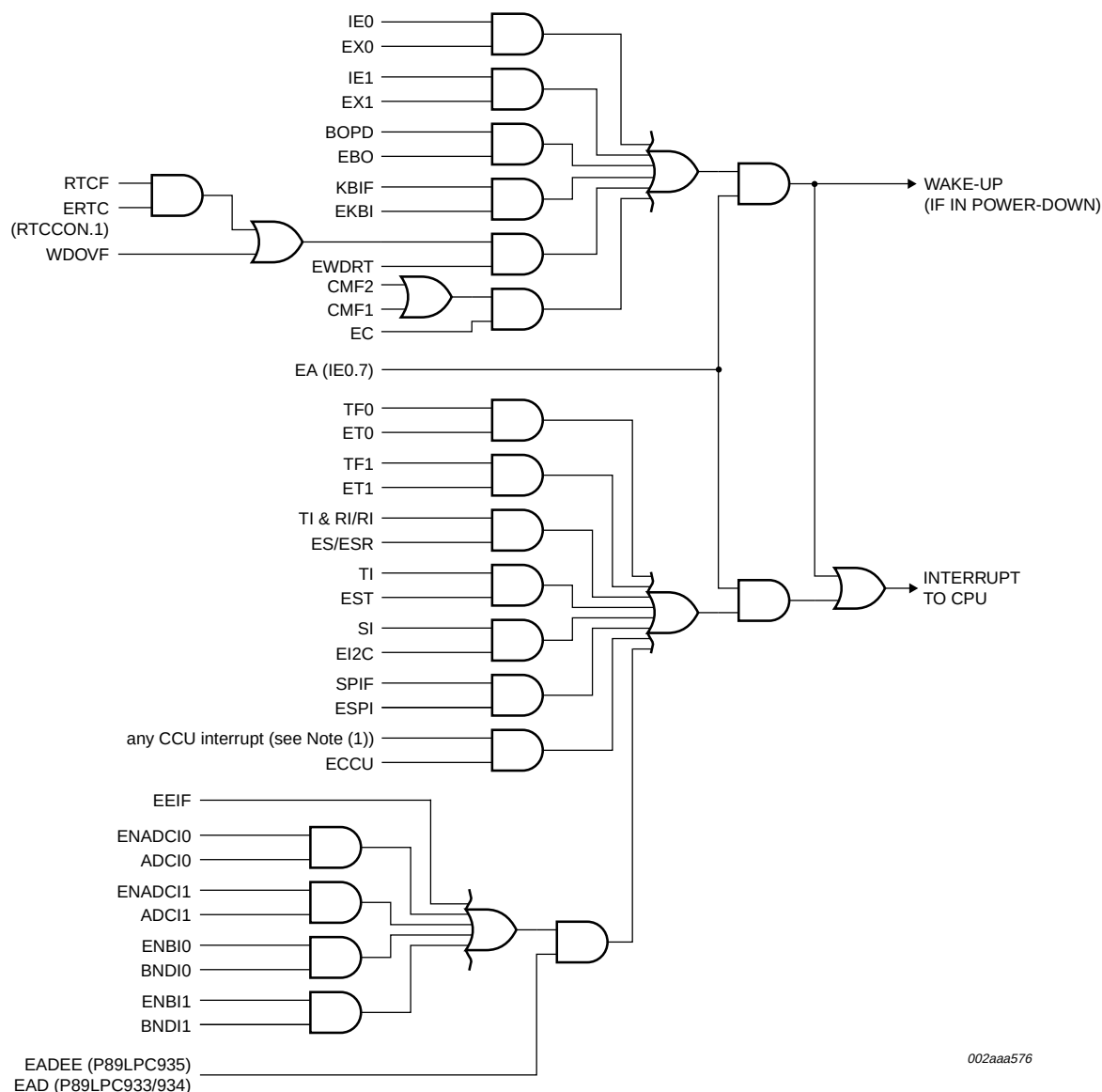
Fig 14. Interrupt sources, interrupt enables, and power-down wake-up sources.
