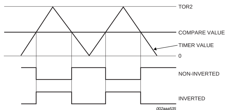
Fig 16. Symmetrical PWM.
