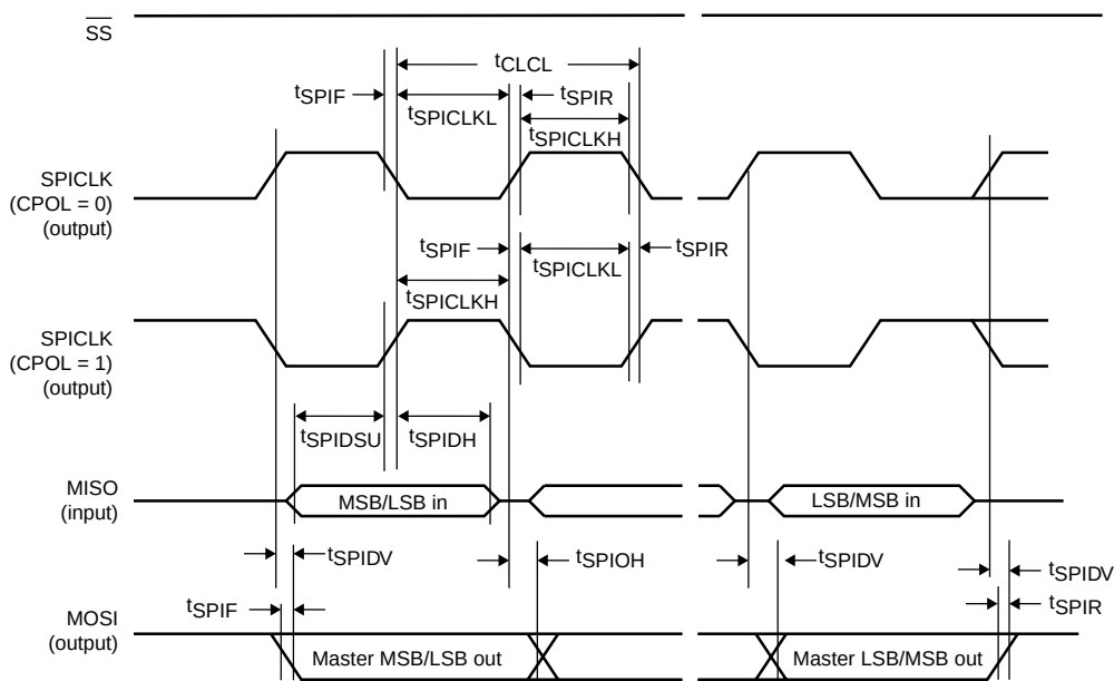
Fig 31. SPI master timing (CPHA = '1')
