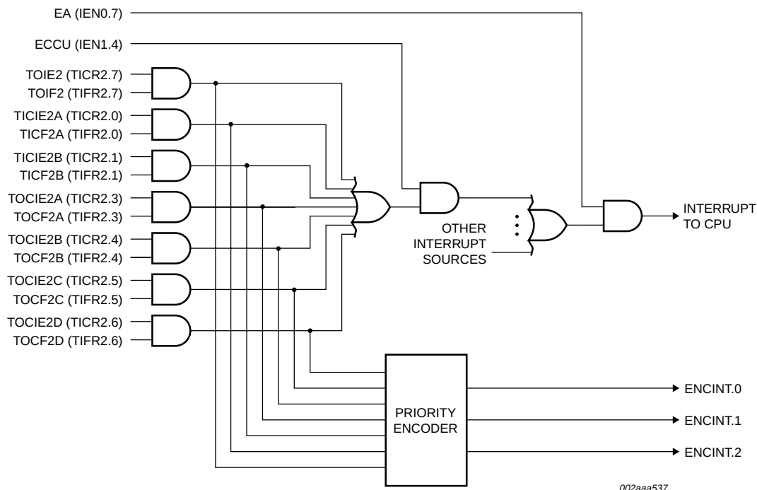
Fig 18. Capture/Compare Unit interrupts.
